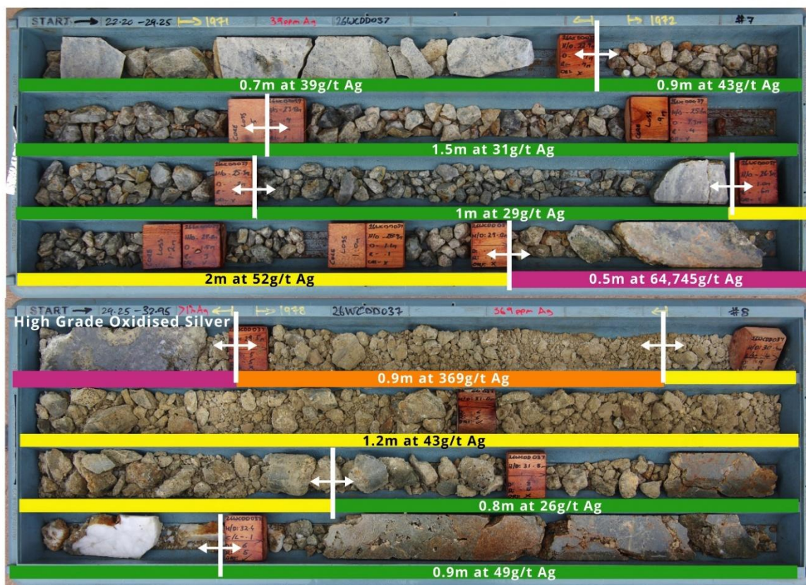
Silver Assay Trace (g/t Ag)
