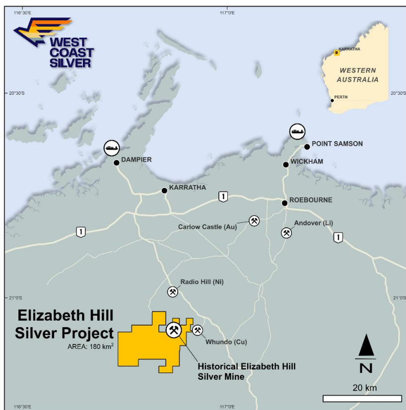
Figure 8. Combined West Coast Silver (WCE), Greentech Metals (GRE) and Alien Metals (AIM Listed: UFO) Tenement Location
