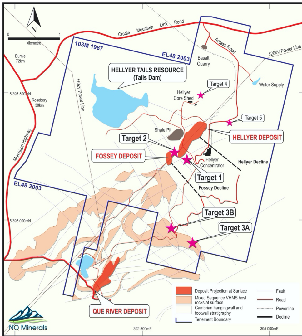
Figure 1: Modelled DHEM Target Locations and Schematic Geology – Hellyer Mine Lease
